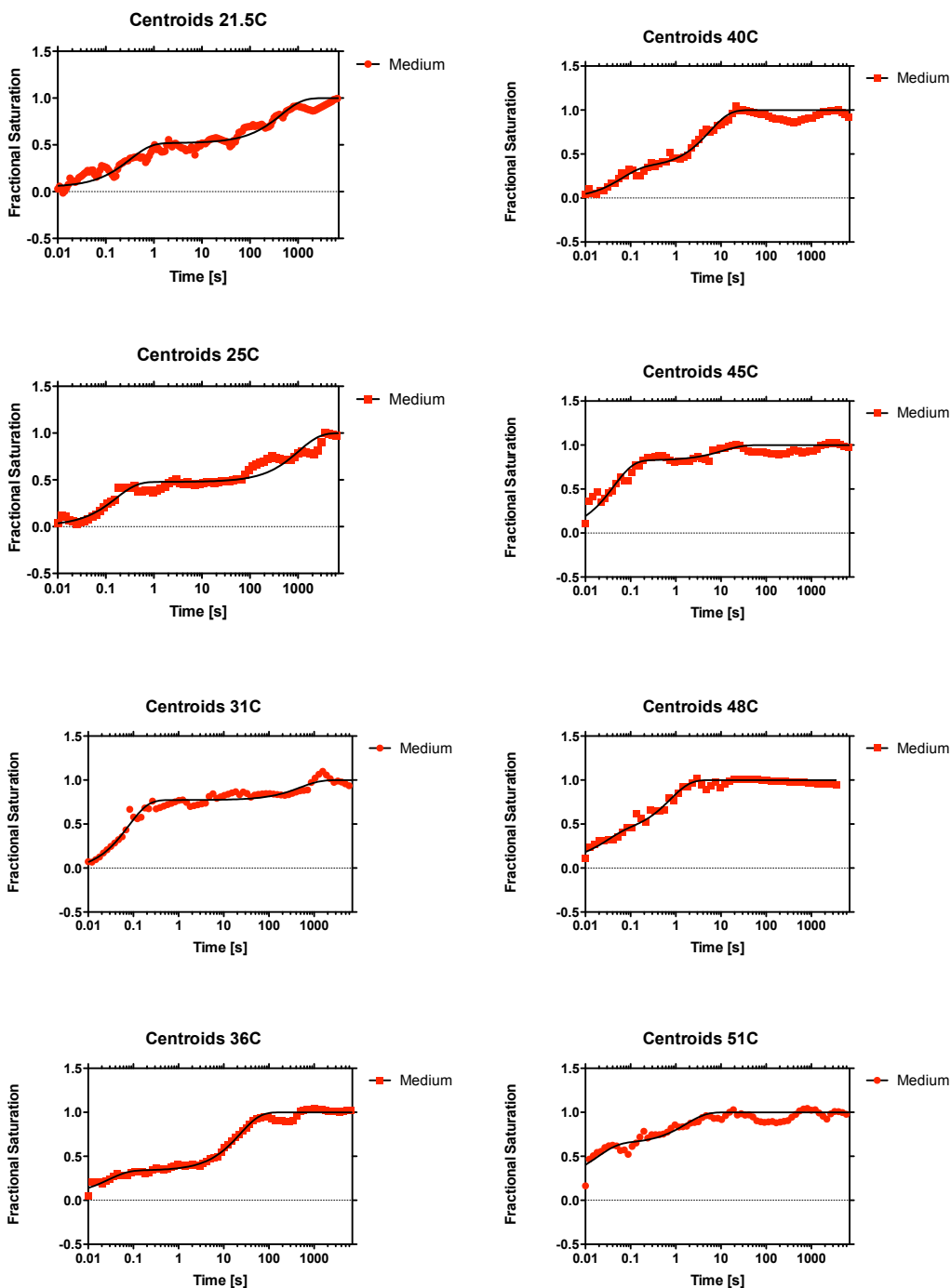
Figure S5. Fitting of the medium cluster. Red dots indicate the raw data of the cluster centroid, the black line shows the bi-exponential fit of the data to equation 3.
