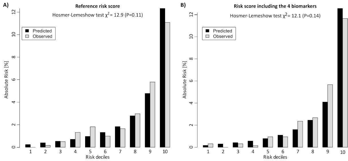
Figure S3. Calibration of risk prediction scores for 5-year all-cause mortality in the FINRISK cohort.
