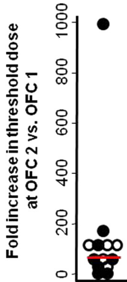
FIG E1. Distribution of the fold increase in threshold dose of peanut protein inducing allergic symptoms for OFC2 compared with OFC1 ( n = 13 ). Open circles indicate group A subjects; solid circles indicate group B subjects. The median response is indicated by the red bar .
