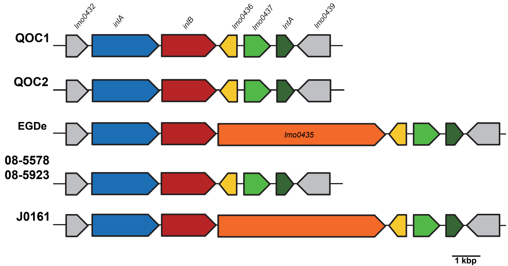
Figure S3: Genomic organization of the inIAB locus in L. monocytogenes serovar 1/2a outbreak strains. Homologous proteins are shown in the same color. L. monocytogenes EGDe locus_tags are indicated in the top row.
