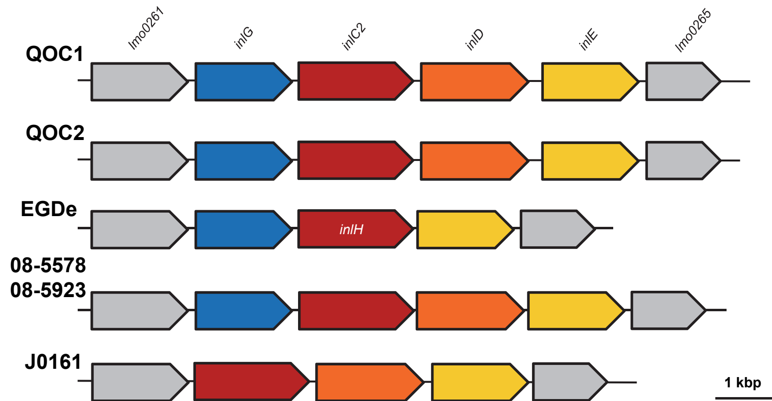
Figure S4: Genomic organization of the inIGHE/C2DE locus in L. monocytogenes serovar 1/2a outbreak strains. Homologous proteins are shown in the same color. L. monocytogenes EGDe locus_tags are indicated in the top row.
