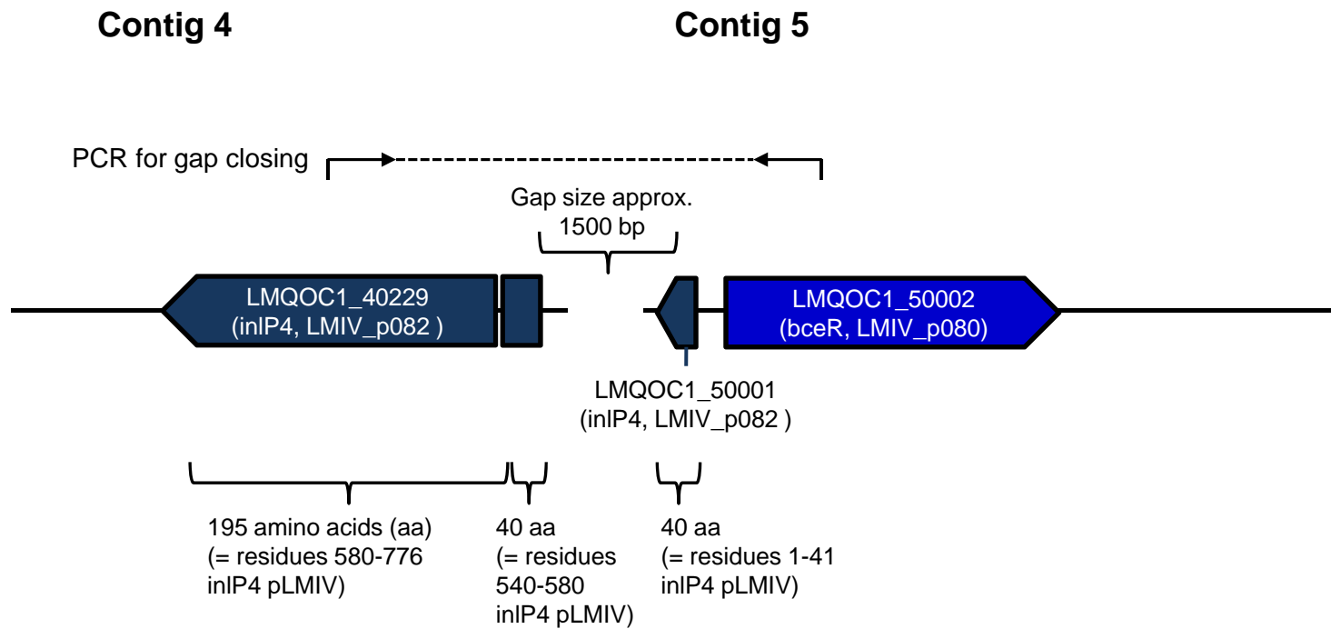
Figure S6: Genomic region surrounding the gap between contig 4 and contig 5 in the L. monocytogenes QOC1 genome.
