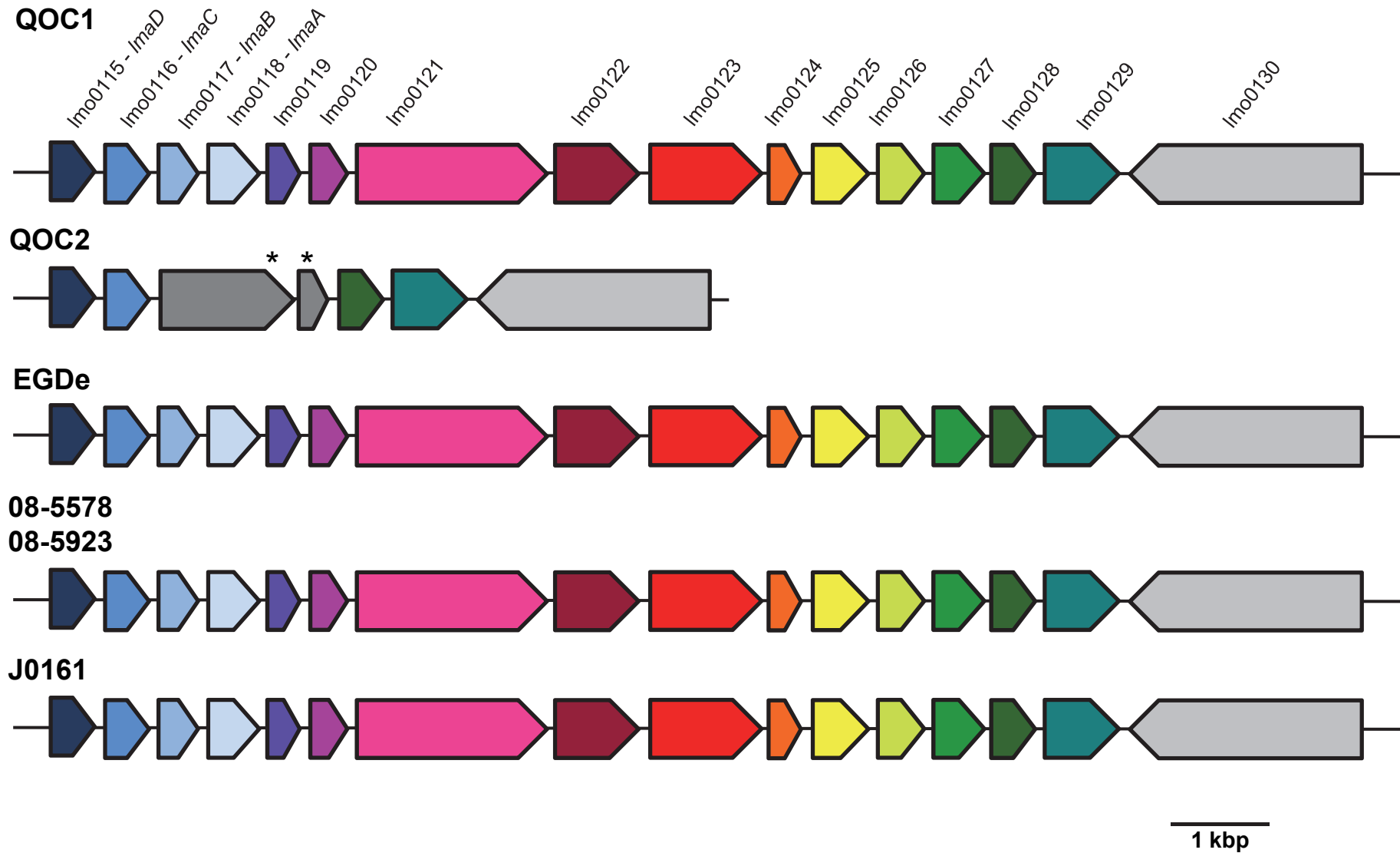
Figure S7: Organization of the monocolin region/lmaDCBA locus in L. monocytogenes serovar 1/2a outbreak strains. Homologous proteins are shown in the same color. L. monocytogenes EGDe locus_tags are indicated in the top row.
