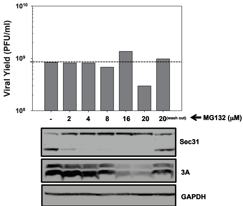
Figure S5. Effect of MG132 on Sec31 levels during PV infection. H1-Hela cells were infected at an MOI of 50 pfu/cell. MG132 was used at varying concentrations and added to the media at the time of infection unless otherwise indicated. Western blots were performed for PV-3A, Sec31, and GAPDH.
