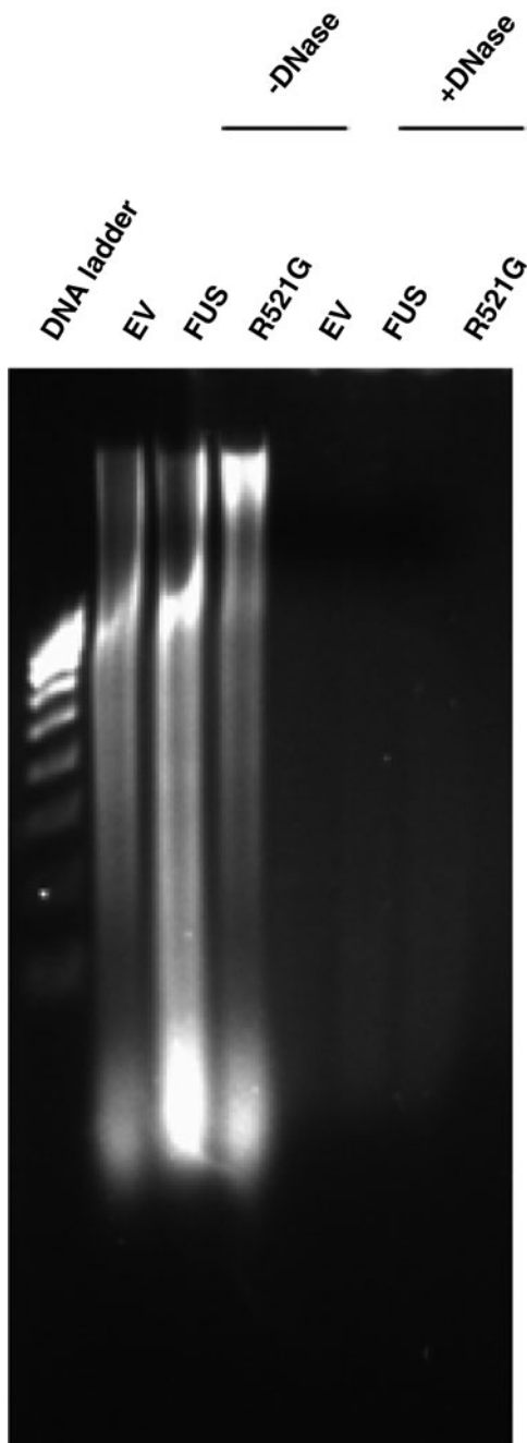
SUPPLEMENTARY FIG. S5. Agarose gel electrophoresis of genomic DNA. Genomic DNA was isolated for the cells after transfection of wild-type or mutant FUS expression vector. Cells were treated with DNase for 30 min, and the DNA samples were resolved in agarose gel electrophoresis.
