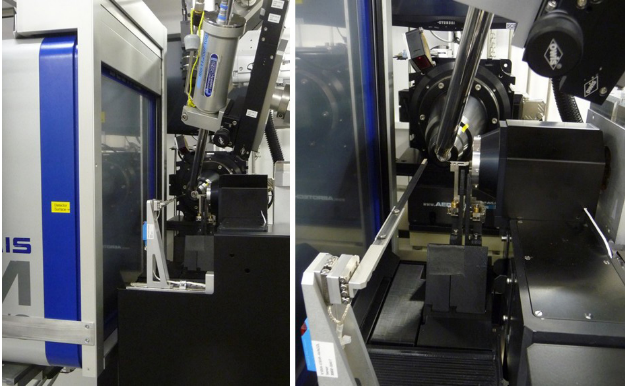
Figure 2 Left: Sample environment with the Pilatus 6M detector with opened protective cover. Right: Sample environment in Data Acquisition state, with retracted illumination and extended beam shaping devices.
