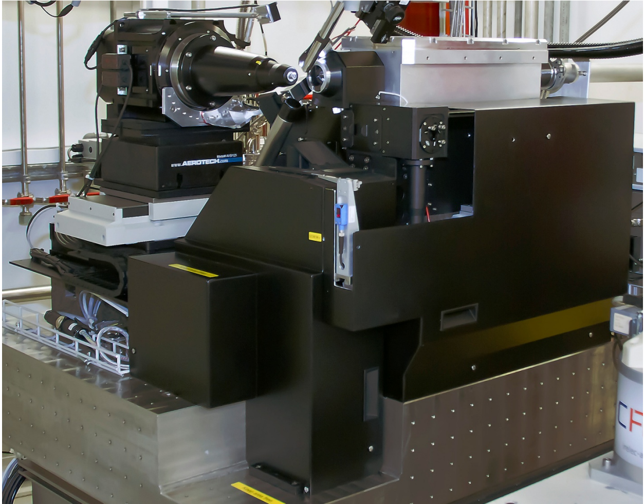
Figure 3 Diffractometer cover close to sample. A two-piece Al-cover protects all cabling and actuators of the diffractometer with the exception of the goniometer at left.
