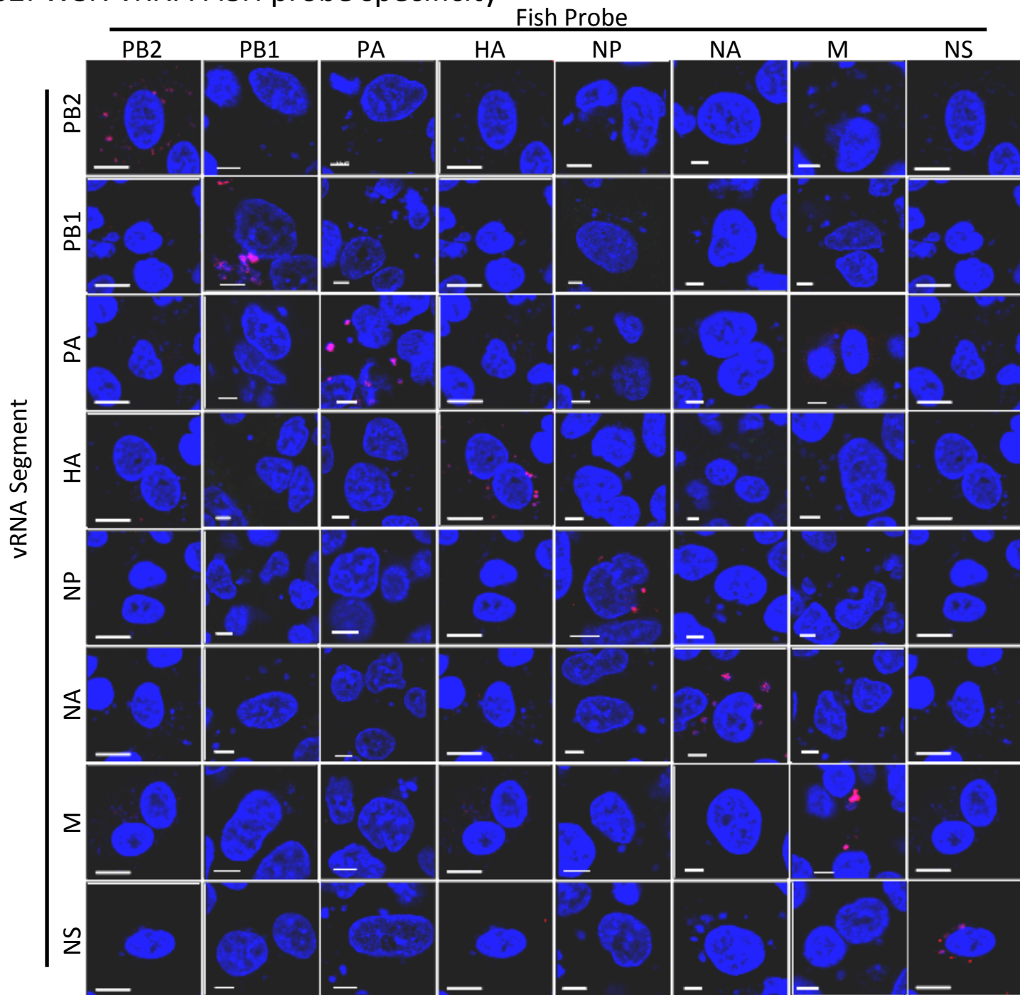
Figure S2: WSN vRNA FISH probe specificity
