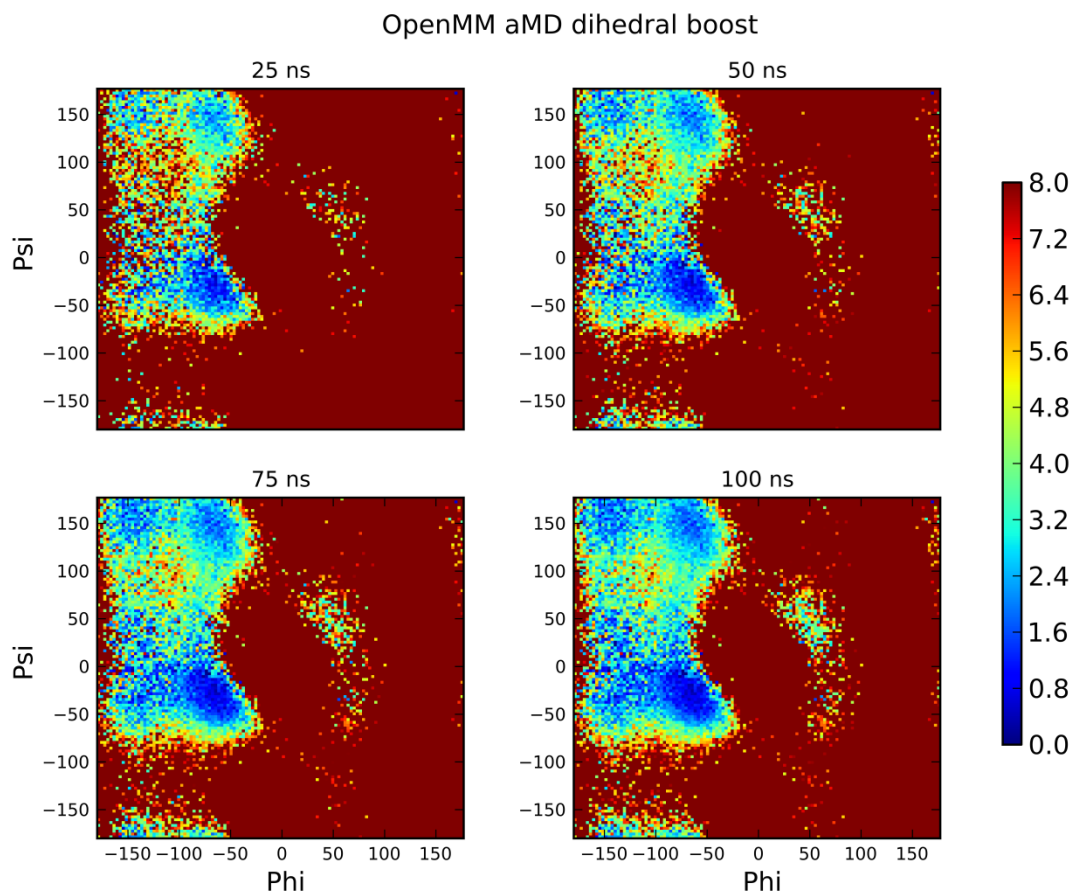
Supplemental Figure 2. Reweighted Phi-Psi free energy maps (in kcal/mol) for alanine dipeptide calculated from dihedral energy boost aMD simulations of length A) 25 ns, B) 50 ns, C) 75 ns, and D) 100 ns.
