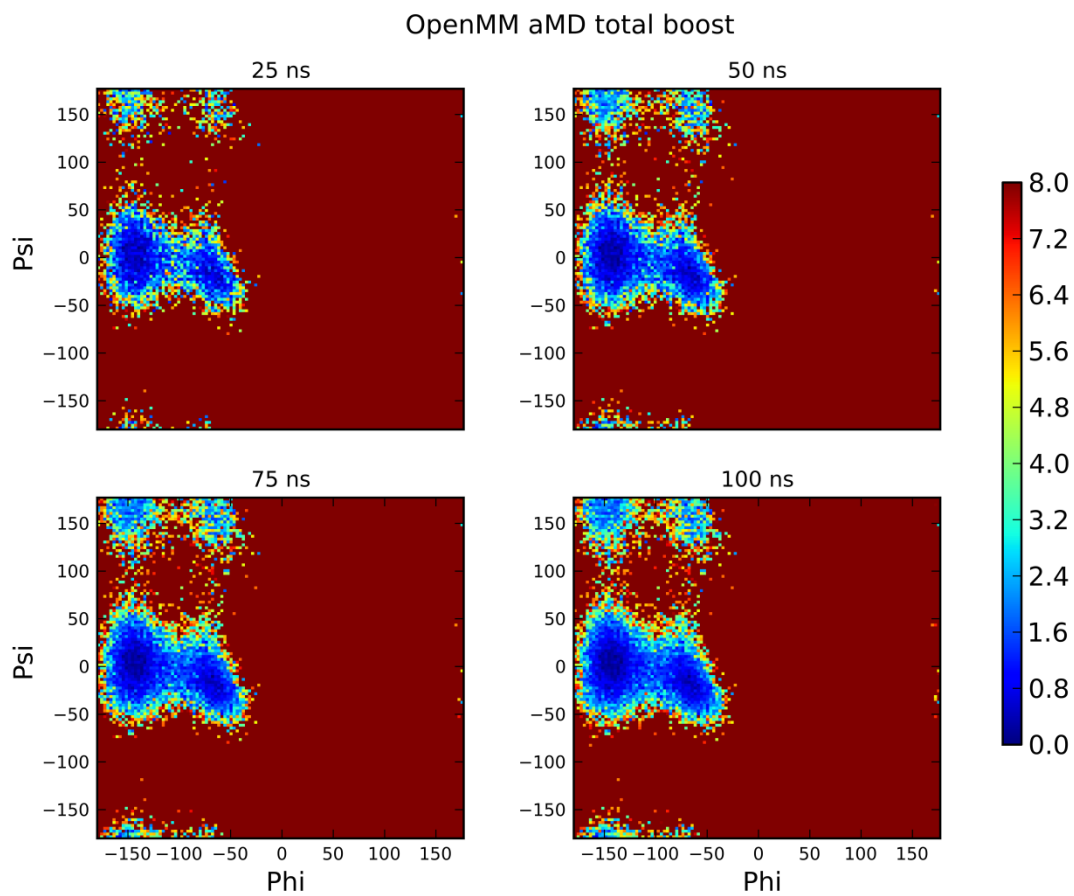
Supplemental Figure 1. Reweighted Phi-Psi free energy maps (in kcal/mol) for alanine dipeptide calculated from total energy boost aMD simulations of length A) 25 ns, B) 50 ns, C) 75 ns, and D) 100 ns.
