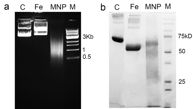
Figure S6. Cleavage with MNP versus released Fe ions. 20 \mu\text{g} MNP were incubated in 50 \mu\text{l} NaAc (0.1M, pH 4.5) for 1 hour at 37°C, and then collected by centrifugation. The supernatant and resuspended MNP were separately mixed with 1% \text{H}_2\text{O}_2 and either 2 \mu\text{g} DNA (a) or 20 \mu\text{g} BSA (b) and incubated to see which was responsible for cleavage. “M” denotes DNA or protein marker, respectively. “C” denotes control with DNA or BSA only. All experiments were repeated in triplicate with representative images shown.
