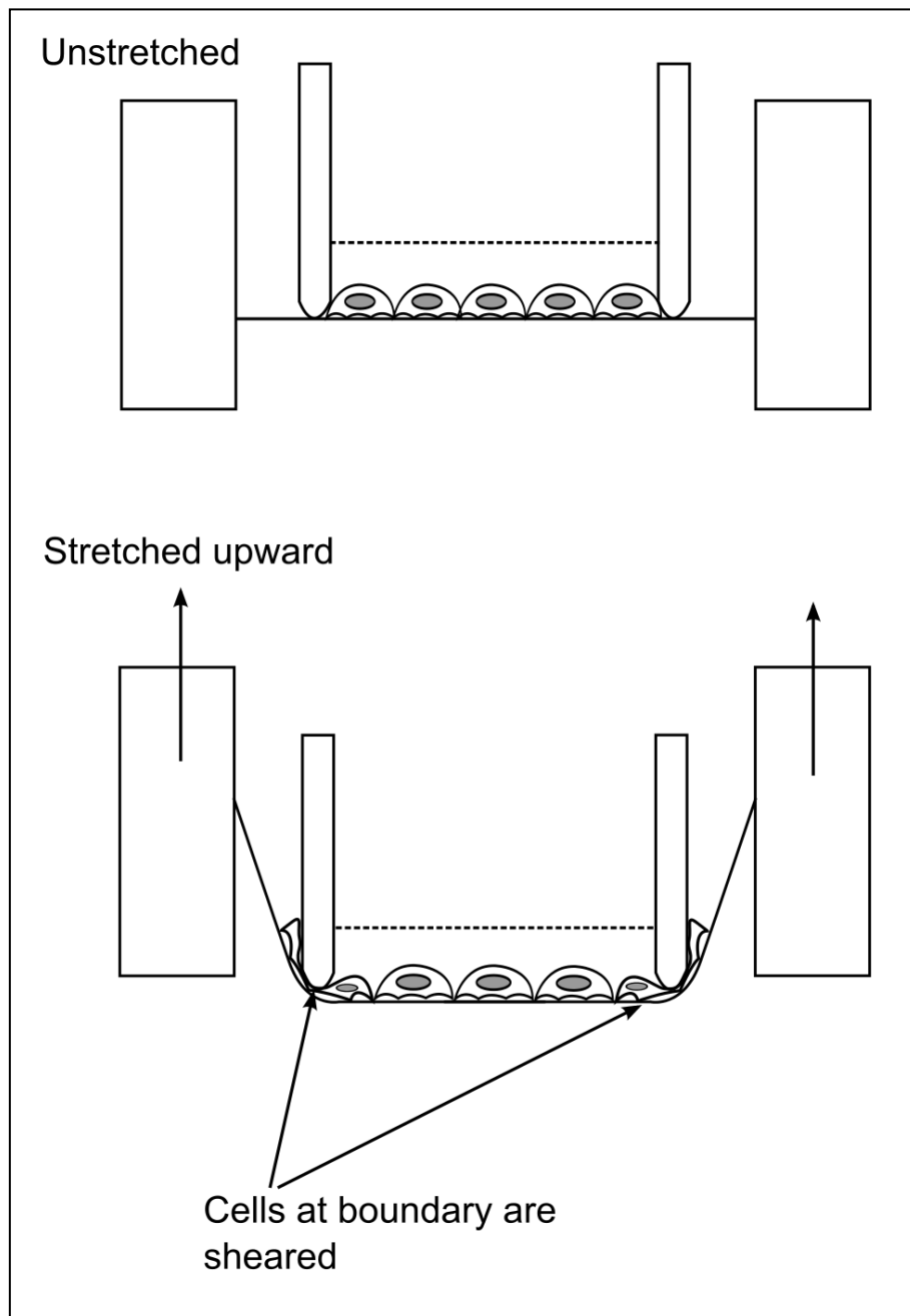
Figure S2. Inverting the configuration of indenter and membrane leads to cell shearing at the boundary. In some of the existing devices, the indenter is placed on the upper surface of the membrane. While a well for cell culture is created by the indenter, cells on the periphery may undergo shearing between the indenter and the membrane upon stretching.
