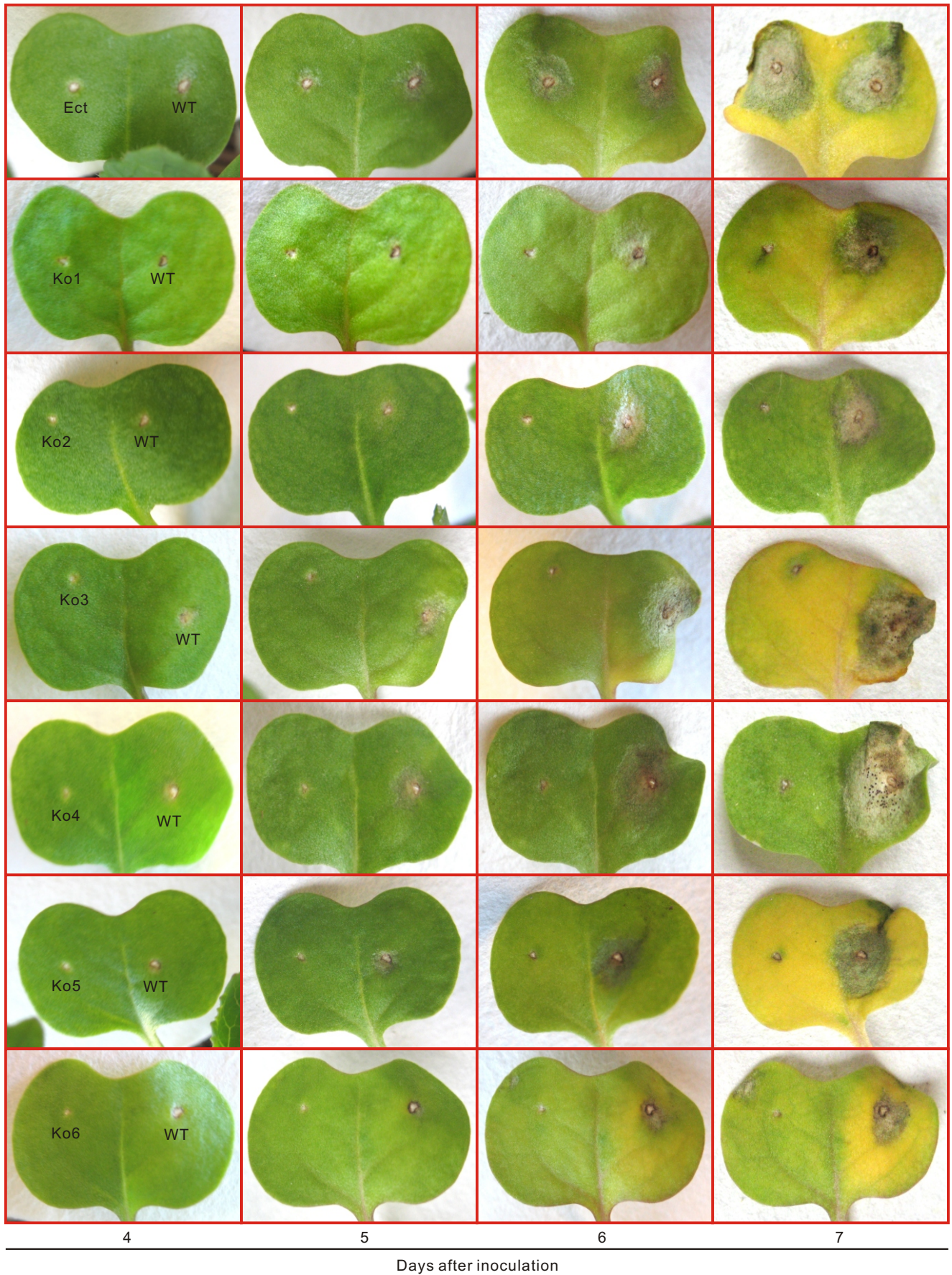
Figure S5. Lesion development on canola cotyledons after inoculated with L. maculans strains.
