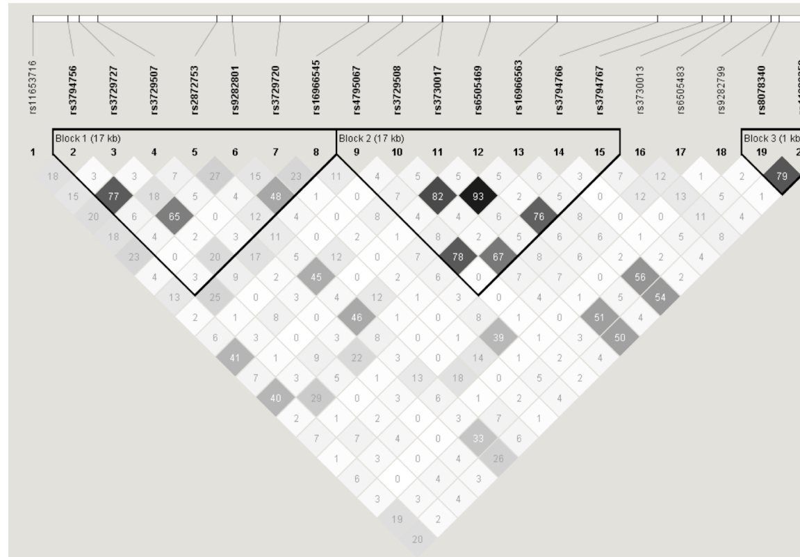
Figure S2. LD map for the tested SNPs in the Angolan population obtained with Haploview 4.2 (values represent pairwise r^2 ).
