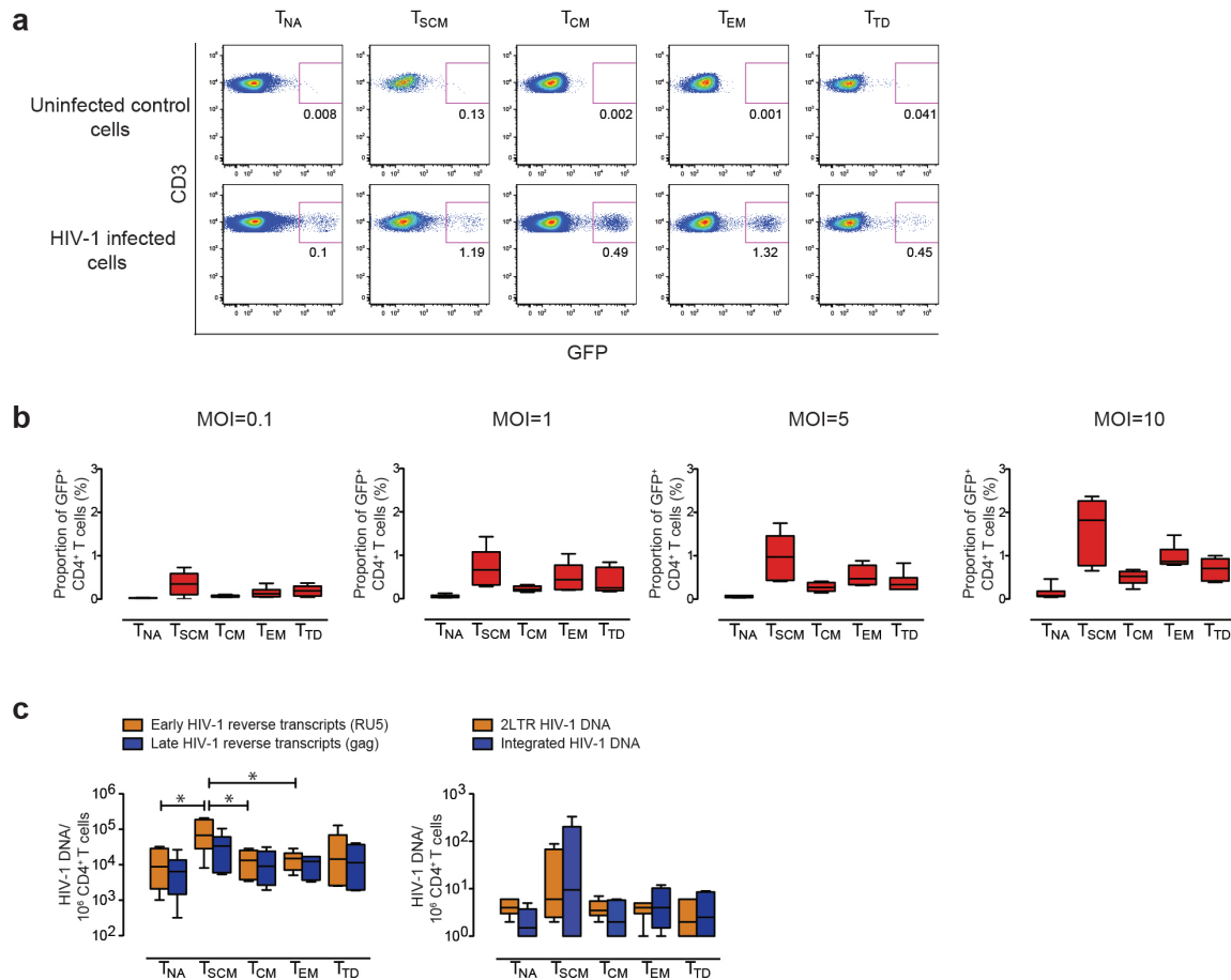
Supplementary Figure 3: Susceptibility of CD4 + T SCM cells to ex-vivo infection with HIV-1. (a): Representative flow cytometry panels reflecting the proportion of HIV-1 infected cells in indicated CD4 + T cell subsets after infection with GFP-encoding, R5-tropic HIV-1. (b): Proportion of GFP + cells within indicated CD4 + T cell populations after ex-vivo infection of unstimulated PBMC with GFP-encoding VSV-G-pseudotyped HIV-1 at the indicated MOI. Experimental results from n=6 study subjects are shown. (c): Quantitative analysis of early/late reverse HIV-1 transcripts, chromosomally integrated HIV-1 DNA and 2-LTR HIV-1 DNA in indicated CD4 + T cell subsets after infection with a VSV-G pseudotyped HIV-1 virus. Data from n=8 study subjects are shown. (b-c): Significance was tested using Wilcoxon rank sum tests followed by Bonferroni correction for multiple comparisons (*reflects p<0.05).
