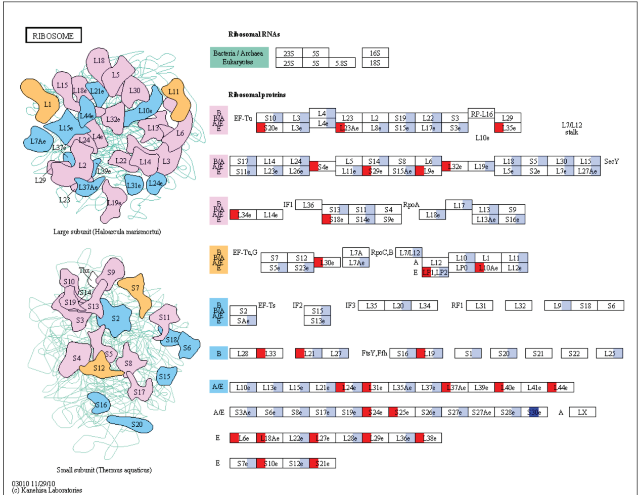
Figure S3. KEGG pathway analysis shows that in the PL-EL comparison, 29/30 significantly differentially expressed ribosomal proteins identified in our mRNA-seq data were up-regulated in the EL population. In this figure, the background non-differentially expressed proteins are shown in light blue, whereas those that are up- or down-regulated are shown in red and dark blue, respectively.
