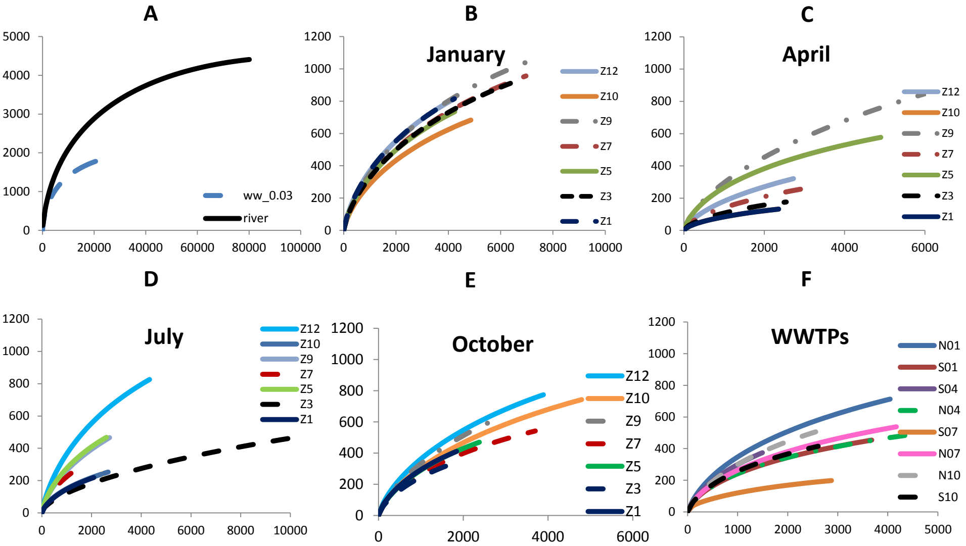
Figure S1 Rarefaction analysis for pooled and individual samples of river and wastewater treatment plant at 97% cutoff level.
