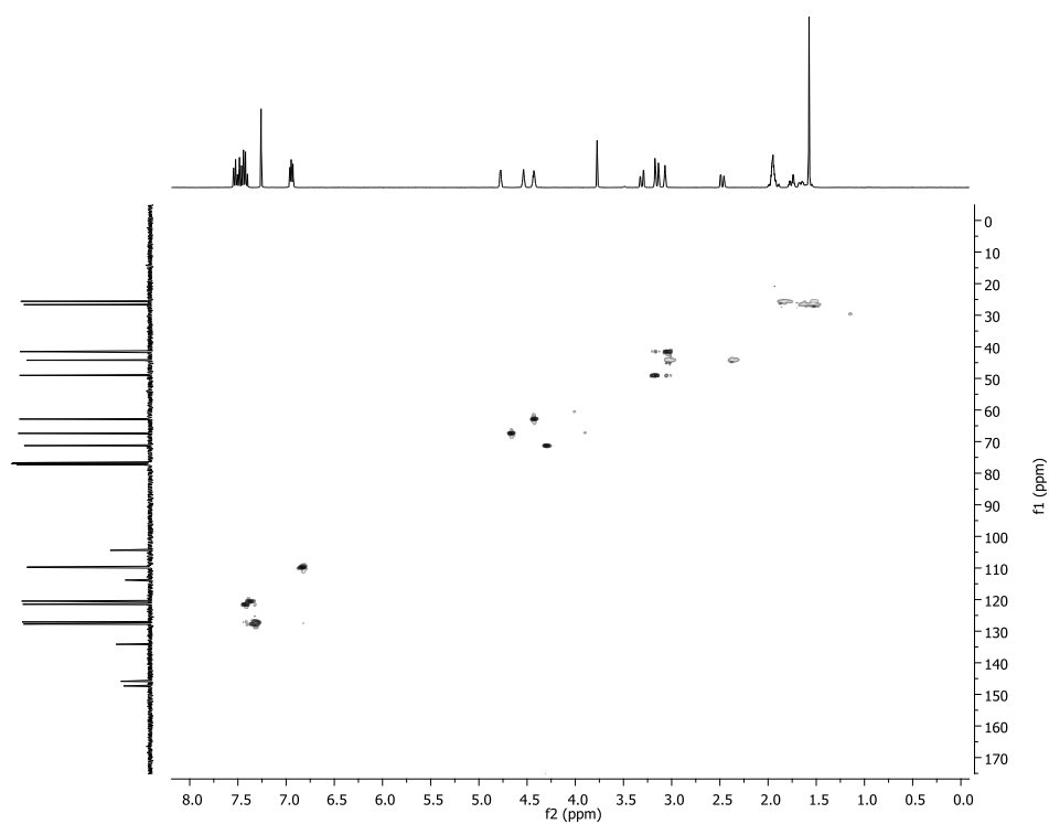
Figure S14. HSQC Spectrum of Rhytidone B (2) in \text{CDCl}_3 .
