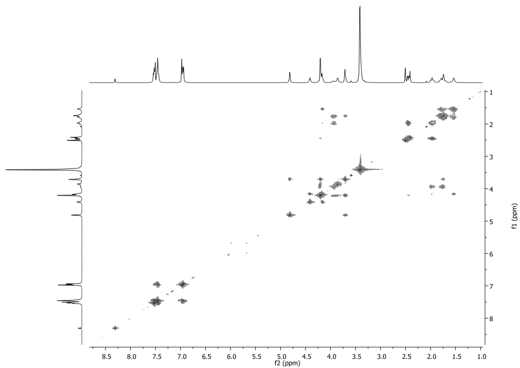
Figure S4. HSQC Spectrum of Rhytidone A (1) in \text{DMSO-}d_6 .
