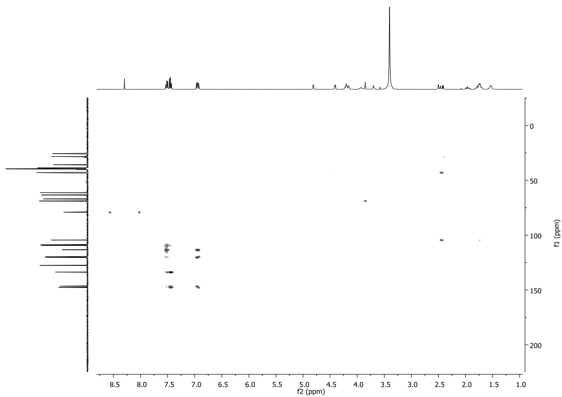
Figure S6. ^1\text{H} NMR Spectrum of Compound 1a in \text{CDCl}_3 .
