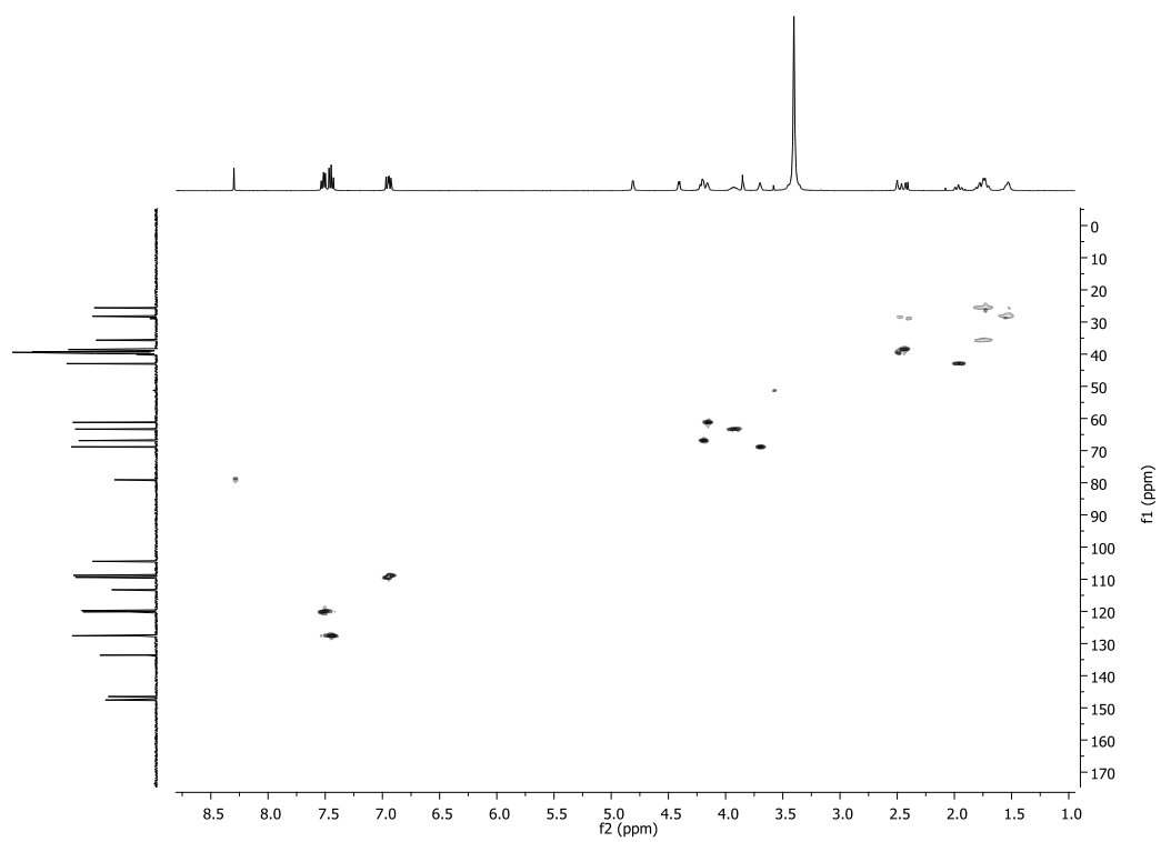
Figure S4. HSQC Spectrum of Rhytidone A (1) in \text{DMSO-}d_6 .
