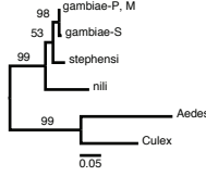
2R-AGAP003327
