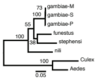
X-AGAP00064
