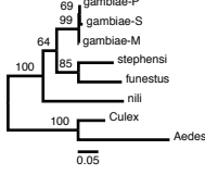
2R-AGAP004028
