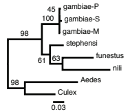
2R-AGAP002019
