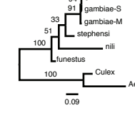
3R-AGAP007903
