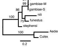
2L-AGAP007504
