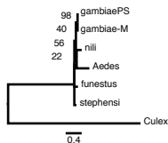
X-AGAP000776
