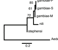
2R-AGAP013533
