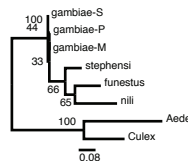
2R-AGAP001287
