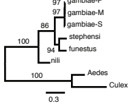
3L-AGAP010267
