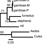
3L-AGAP010567
