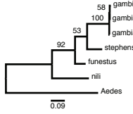
2R-AGAP003584
