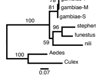
2L-AGAP005851
