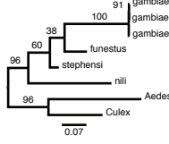
2R-AGAP004486
