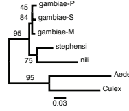
2R-AGAP003328
