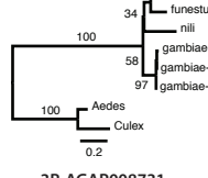
3R-AGAP008731
