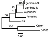
2L-AGAP006783
