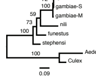
2L-AGAP007069
