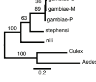
2L-AGAP005778
