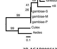
3R-AGAP009512
