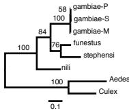
2R-AGAP001762
