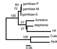
2R-AGAP001700
