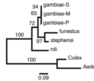
2R-AGAP002424
