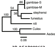
3R-AGAP008652
