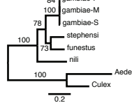
2L-AGAP005542
