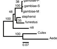
2R-AGAP004199
