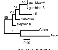
3R-AGAP009133
