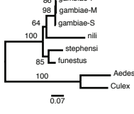
2L-AGAP005279
