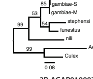
3R-AGAP010007
