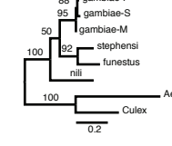
2L-AGAP006531
