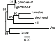
2L-AGAP007131
