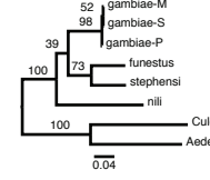
2R-AGAP003397
