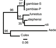
2L-AGAP007068
