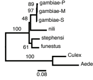
2R-AGAP003043
