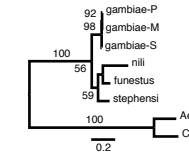
2R-AGAP002933
