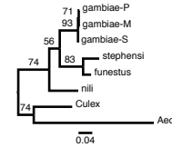
2R-AGAP002790
