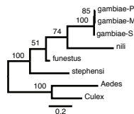
X-AGAP00521
