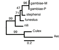
2L-AGAP006209
