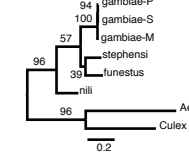
2L-AGAP005014
