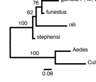
2L-AGAP004699
