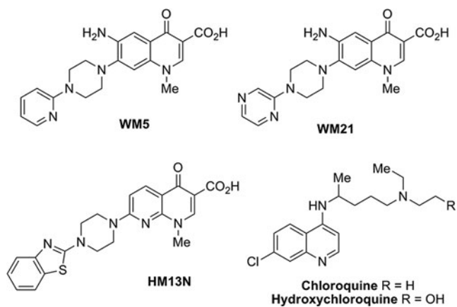
SUPPLEMENTARY FIG. S1. Structure of the three studied 6-desfluoroquinolone compounds (6-DFQs), chloroquine (CQ), and hydroxychloroquine (HCQ). The structures of the three 6-DFQs tested in this study, WM5, WM21, and HM13N, are shown in comparison with CQ/HCQ.
