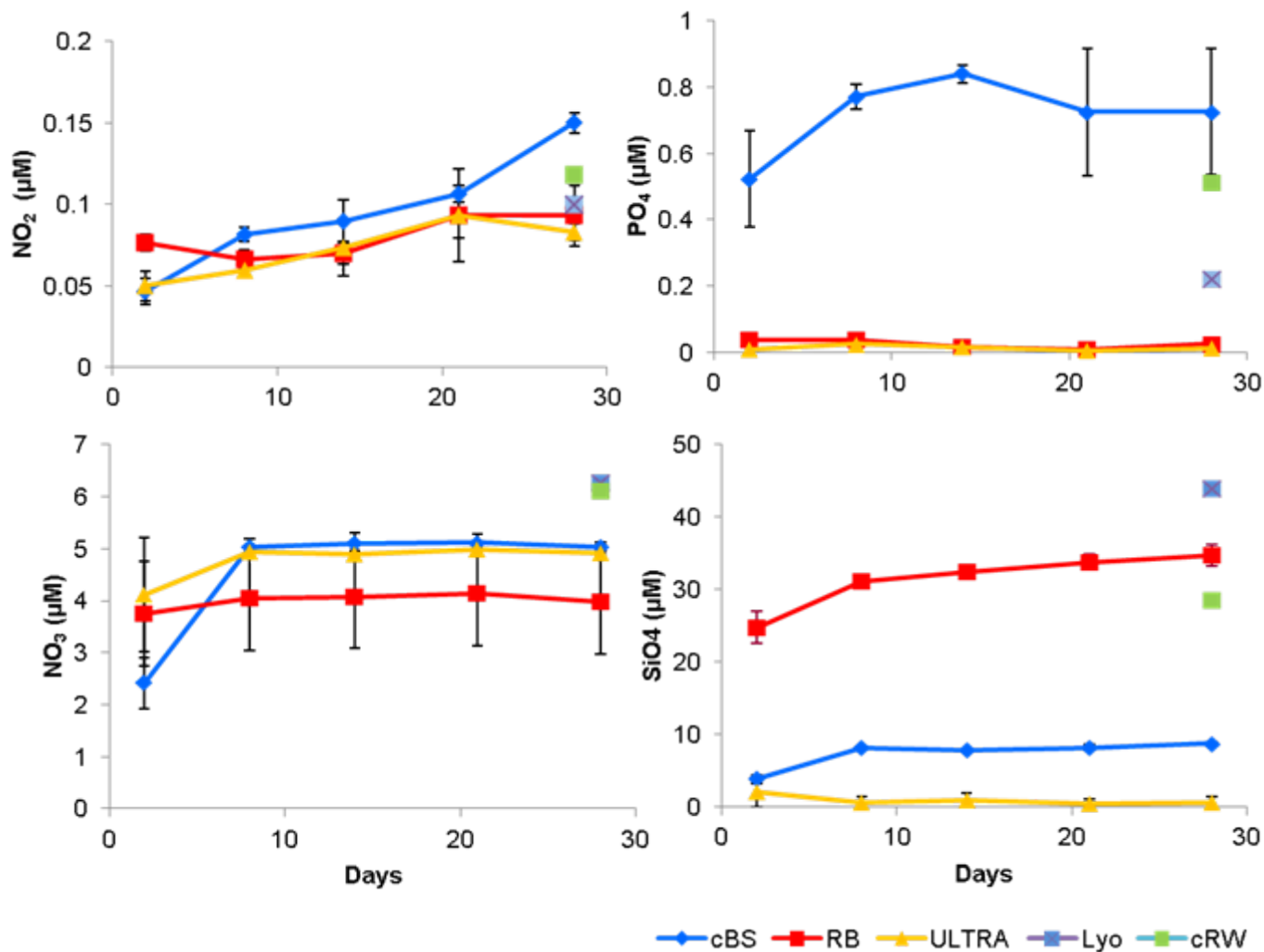
Figure S3. Nutrients measured during the experiment. Shown is the average concentration of three independent replicated mesocosms: (A) NO 2 , (B) PO 4 , (C) NO 3 , (D) SiO 4 . For abbreviation of the treatments see Fig 1.
