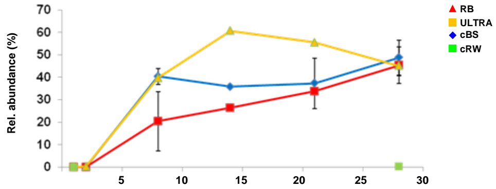
Figure S6. Relative proportion of the Paraperlucidibaca assigned pyrosequencing reads in the mesocosms. Shown is the relative average abundance of three replicated mesocosms. For abbreviation of the treatments see Fig 1.
