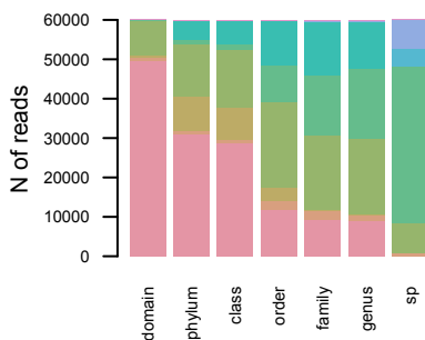
MetaSim 4
