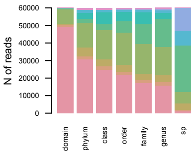
MetaSim 1
