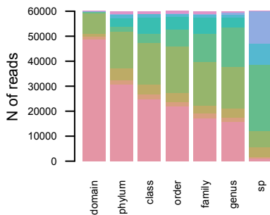
MetaSim 2
