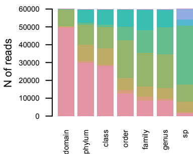
MetaSim 3
