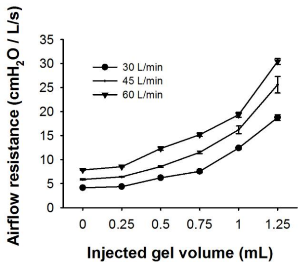
Figure E1 Increase in resistance to airflow in a 7.5 mm ETT by increase of injected gel amount, resembling the biofilm present at extubation. The increase of resistances is more pronounced at higher flows ( p < 0.001 )
