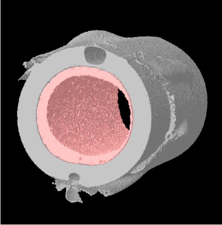
Figure E2 Exemplary 3d-reconstruction of MicroCT scan of an ETT portion. The layer of secretions present on the inner lumen in the cuff portion is highlighted in light red.
