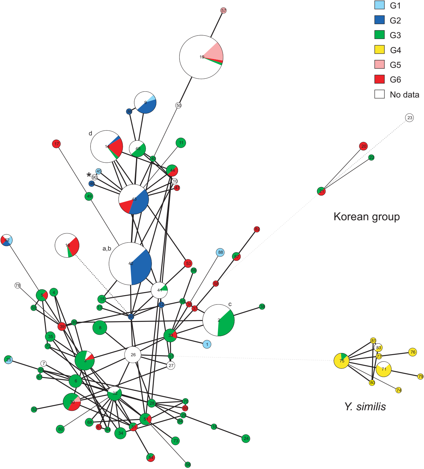
Y. pseudotuberculosis s.s.
