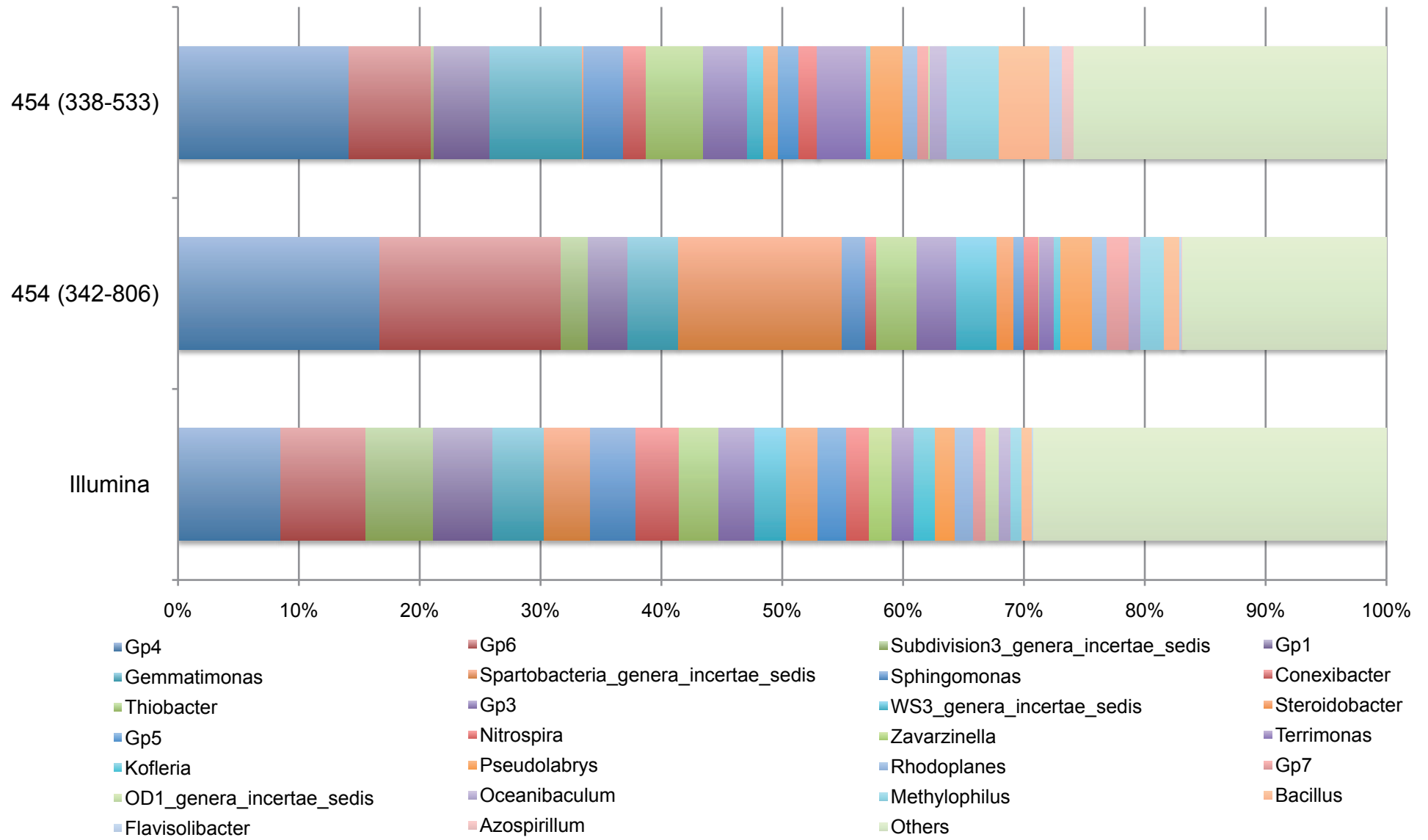
Fig. S3. 16S rRNA-based genus-level taxonomic compositions by the 338F-533R and 342F-806R amplicon sequencing and by the Illumina metagenomic sequencing. The top 26 genera that were found among the top 20 most-abundant genera in the three experiments are represented.
