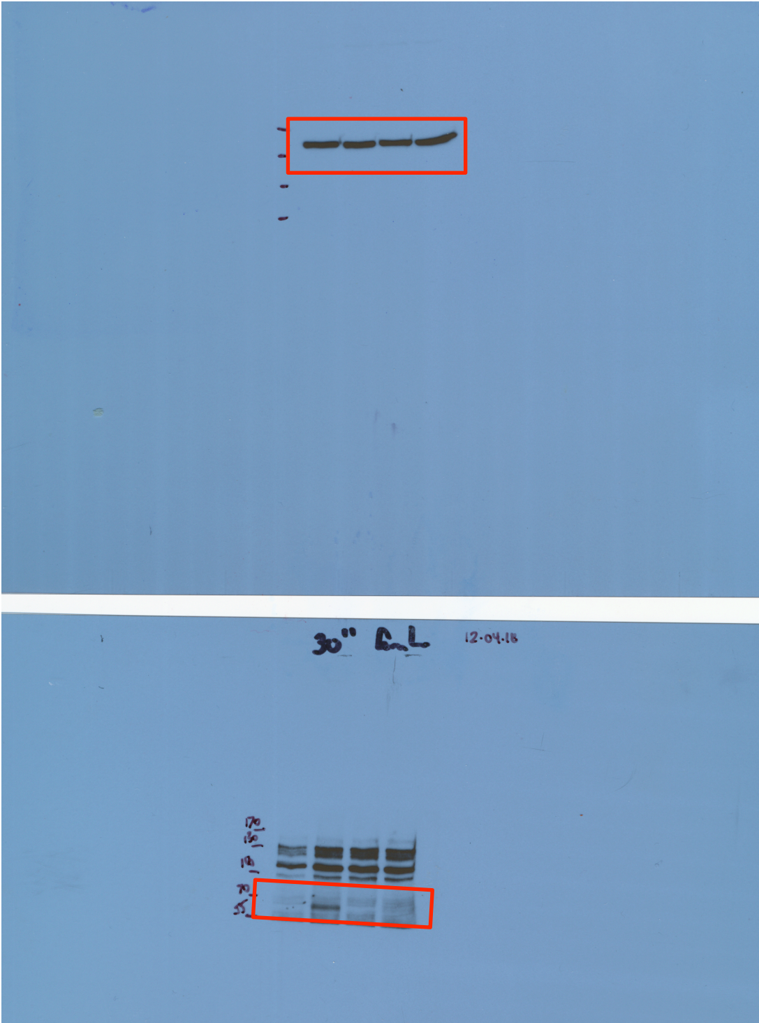
Fig. 5A: immunoblot
