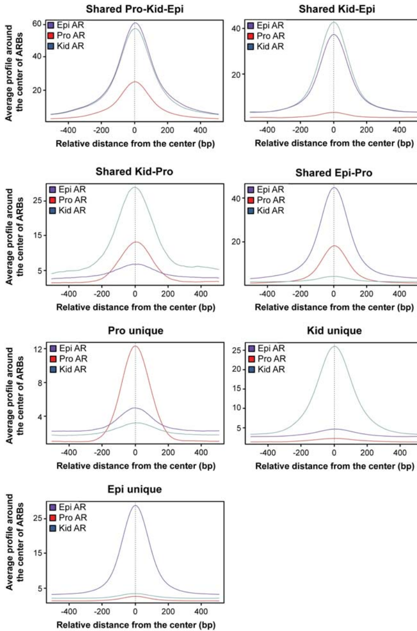
Supplementary Figure S1. Average tag density profiles of AR ChIP-seq reads for receptor-binding events unique to prostate, kidney or epididymis and for those shared in two or three tissues.
