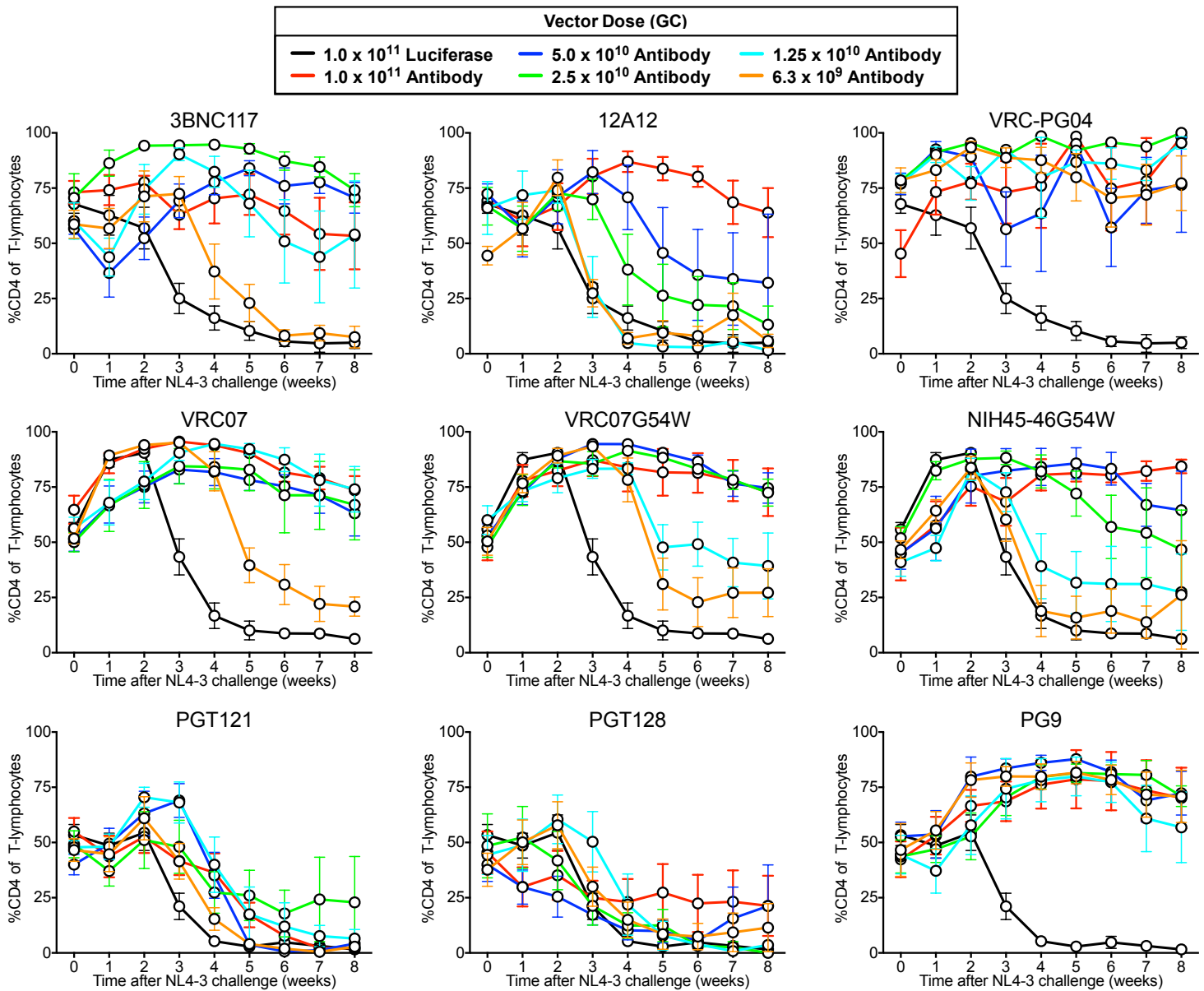
Protection against NL4-3 challenge in vivo by the indicated antibody concentration ( \mu\text{g ml}^{-1} )
