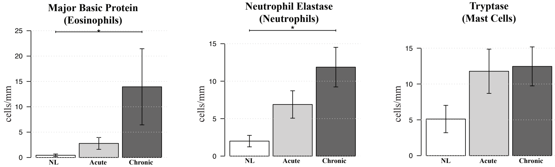
Figure E3. Cell counts of eosinophils, neutrophils and mast cells in non-lesional (NL), acute and chronic AD skin lesions. Cell counts of eosinophils (major basic protein+ cells) and neutrophils (neutrophil elastase+ cells) increased from non-lesional through chronic disease ( P < 0.04 , and P < 0.02 , respectively). * P < .05 , ** P < .01 , and *** P < .001 , ( n = 10 ). Bar plots represent mean \pm SEM.
