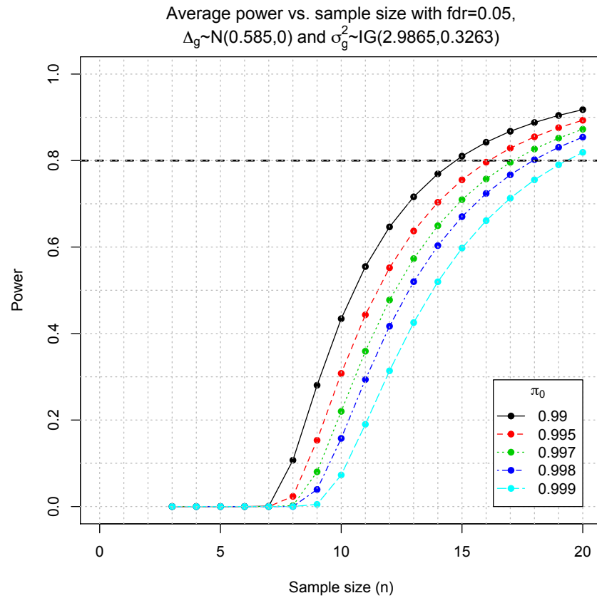
Figure E4. Average power vs. sample size needed to detect differences of 1.5 fold change at 0.05 FDR significance level.
