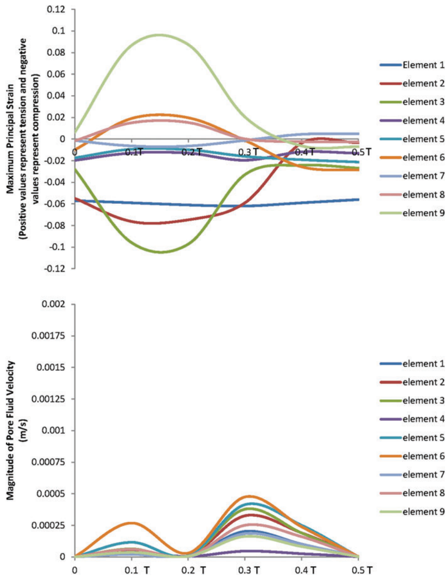
SUPPLEMENTARY FIG. S2. Changes of the maximum principal strain and the pore fluid velocity at nine locations within the scaffolds cross section during the loading cycle in the dynamic interfacial shear alone group (regimen ii). ( T is the period of the loading cycle.)
