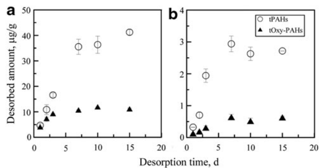
SUPPLEMENTARY FIG. S1. Desorption kinetics of total PAHs and total oxy-PAHs to HLB resin from (a) feed soil and (b) treated soil removed from the bioreactor 1 day after feeding, using the dialysis-tubing desorption method described in the text.
