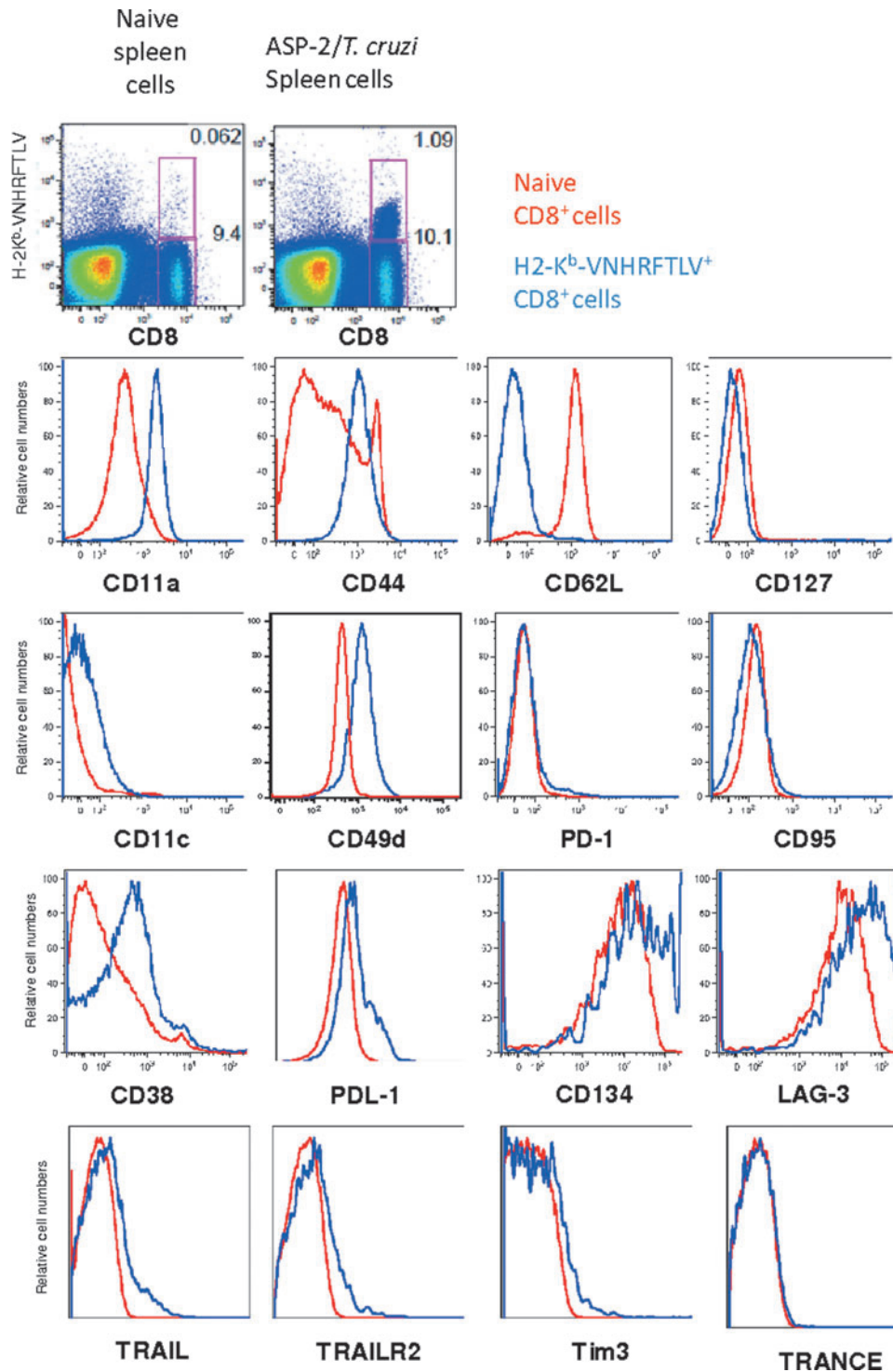
SUPPLEMENTARY FIG. S1. Phenotype of specific splenic CD8 + T cells after infectious challenge with T. cruzi in mice vaccinated with the heterologous prime-boost vaccination regimen. C57BL/6 mice were immunized and challenged as described in the legend of Fig. 1. Fourteen days after the challenge, pools of splenic cells from four mice were stained with anti-CD8, H-2K b -VNHRFTLV, and antibodies to the indicated surface markers. The red and blue lines denote the naïve CD8 + cells and H-2K b -VNHRFTLV CD8 + cells, respectively.
