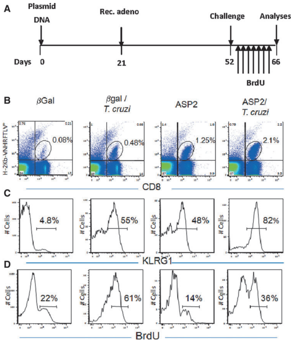
SUPPLEMENTARY FIG. S4. Limited proliferation of specific CD8 + T cells after challenge in mice that have been previously vaccinated with the heterologous prime-boost regimen. (A) GzmBCreERT2/ROSA26YFP transgenic mice were immunized, challenged, and treated as depicted. The mouse groups were the same described in the legend of Fig. 1. (B) Splenic cells were collected at day 66 and stained with anti-CD8 and H-2K b -VNHRFTLV. (C) CD8 + H-2K b -VNHRFTLV + cells were stained with anti-KLRG1. (D) CD8 + H-2K b -VNHRFTLV + cells were stained with anti-BrdU. Results represent pools of four mice per group.
