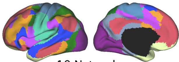
10 Networks
