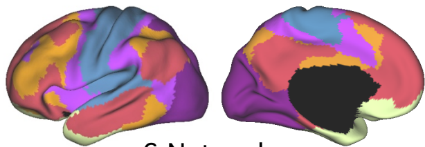
6 Networks
