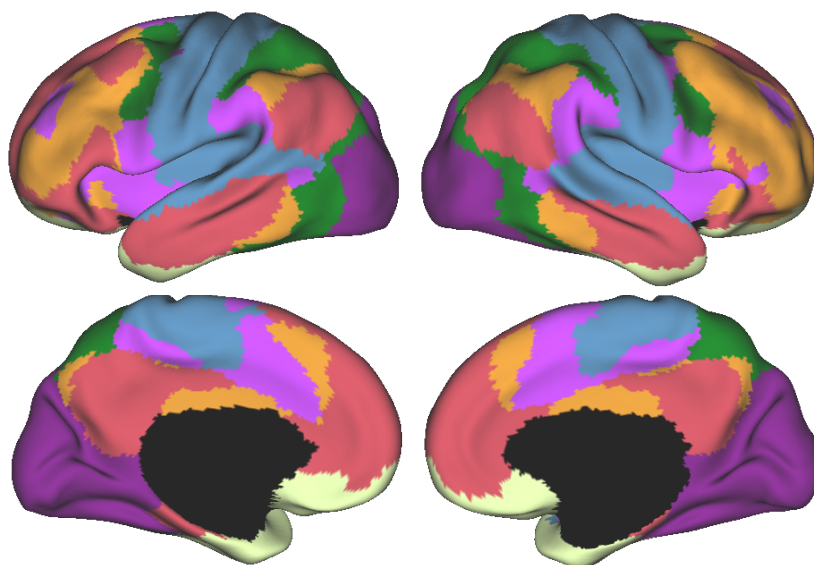
7 Networks
