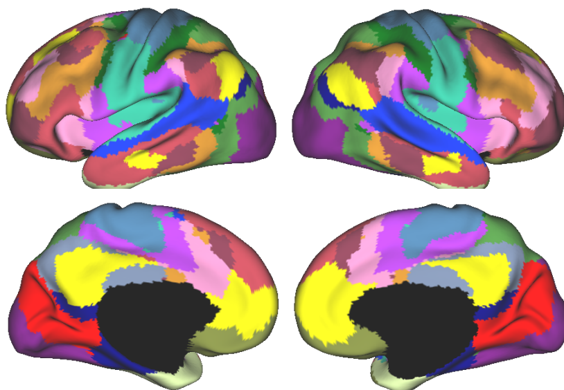
17 Networks
