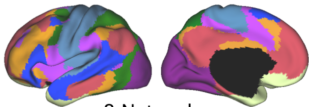
8 Networks
