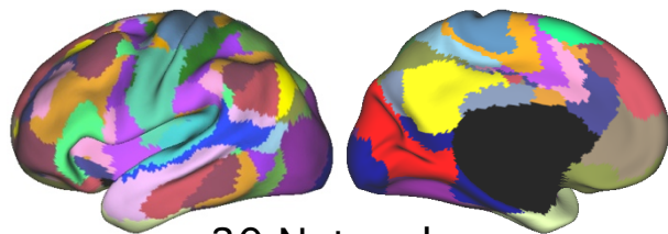
30 Networks
