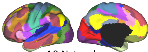
18 Networks
