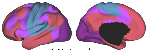
4 Networks
