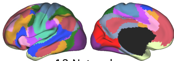
12 Networks
