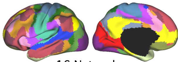
16 Networks
