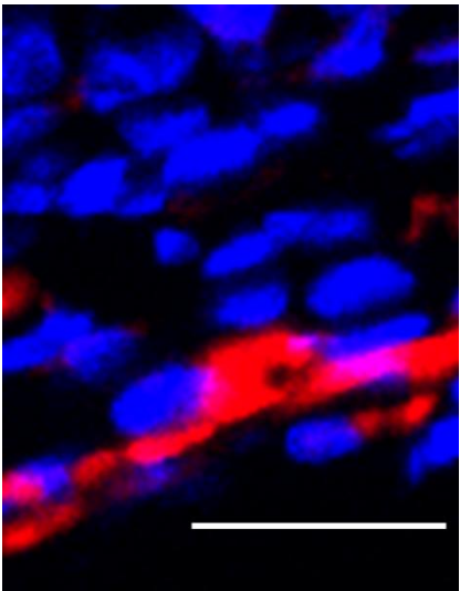
HO-1
