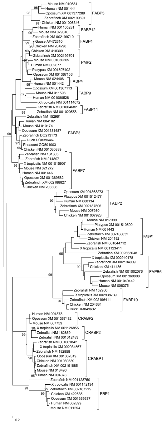
Supplementary Figure S1. Neighbor-joining tree based on JTT + gamma distance ( \alpha = 3.99 ). Numbers on branches are confidence levels of the interior branch test; only values \geq 95\% are shown.
