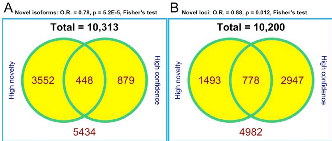
Figure S2. High novelty and high confidence novel isoforms and loci
