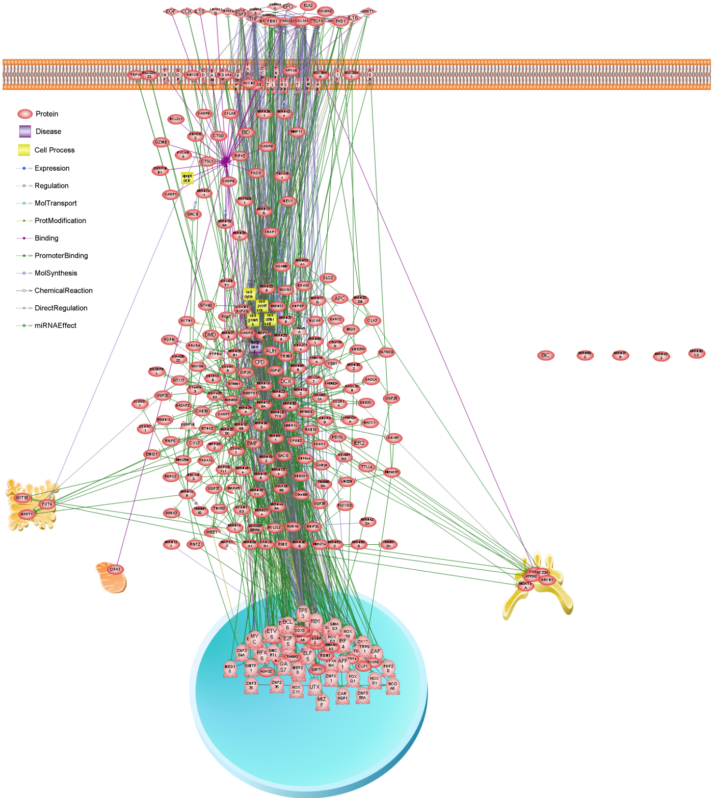
Figure S4 Network of common altered microRNAs in variety of cancers. Network was constructed using pathway studio 9 software (shortest path algorithm). This network comprises 322 entities and 1041 relations and various type of transcription factors , protein kinases , small molecules , mrnas and mirnas serve as either validated or putative regulators.
