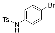
N -(4-bromophenyl)-4-methylbenzenesulfonamide
