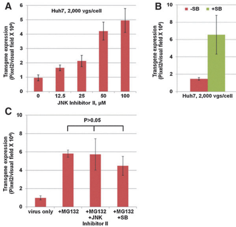
SUPPLEMENTARY FIG. S1. Effect of serine/threonine kinase inhibitors on scAAV3 vector-mediated EGFP expression in Huh7 cells. Cells were transduced with scAAV3 vectors in the presence of increasing amounts of JNK inhibitor II ( A ), 12.5 \mu\text{M} p38 MAPK inhibitor (SB) ( B ), and 5 \mu\text{M} MG132 alone, or with 50 \mu\text{M} JNK Inhibitor II or 12.5 \mu\text{M} p38 MAPK inhibitor ( C ). Transgene expression was determined by fluorescence microscopy 72 hr post-transduction and assessed as total area of green fluorescence (pixel 2 ) per visual field (mean \pm SD).
