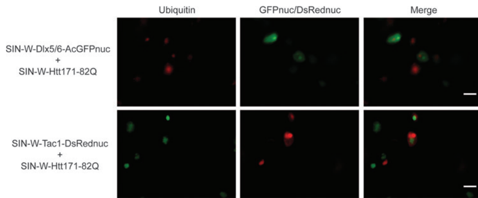
SUPPLEMENTARY FIG. S1. Effect of huntingtin overexpression on the transcriptional activity of the promoters. Double staining showing the formation of Htt aggregates labeled with ubiquitin and co-localization with LV-Dlx5/6 and LV-Tac1 expressing the reporter genes. Scale bar = 10 \mu m.
