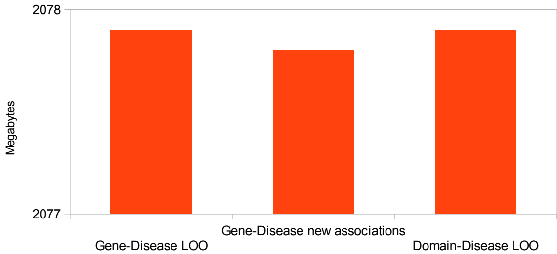
Memory usage
