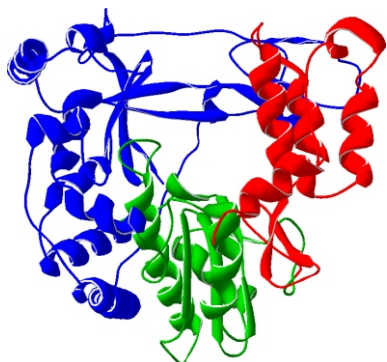
NORV
