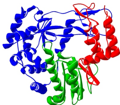
NORV
