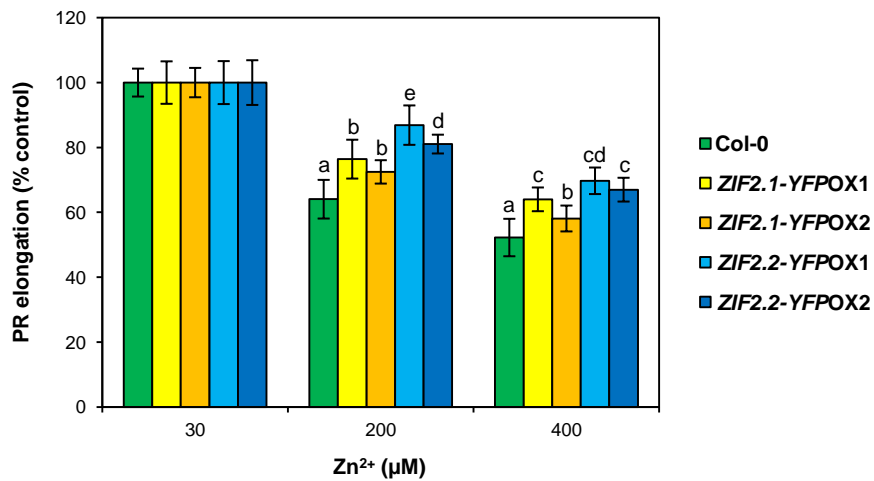
Figure S12 Phenotype of Arabidopsis ZIF2.1-YFP and ZIF2.2-YFP overexpression lines. Effect of Zn toxicity on PR elongation of wild type (Col-0) and ZIF2.1-YFP or ZIF2.2-YFP overexpression lines ( ZIF2.1-YFPOX1-2 or ZIF2.2-YFPOX1-2 ) seedlings. Results are representative of two independent experiments and values represent means \pm SD ( n=16 ). Different letters indicate statistically significant differences between genotypes under each condition ( P<0.05 ; Student's t -test).
